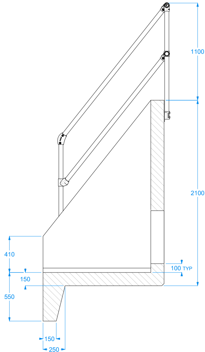
VIEW: SECTION X-X
