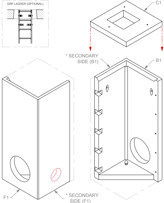
VIEW: ISOMETRIC
