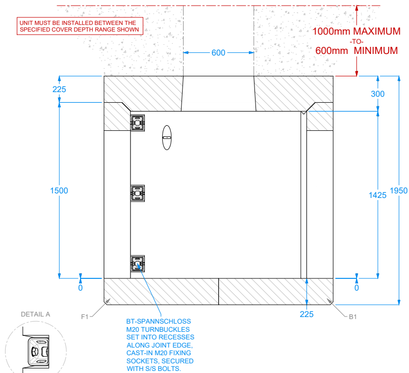
VIEW: SECTION X-X
