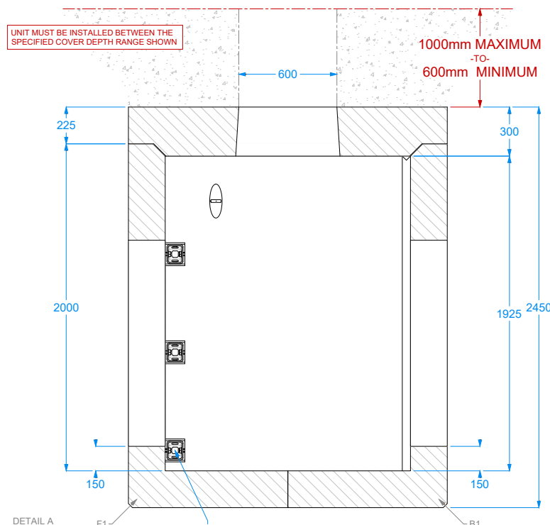
DETAIL A
