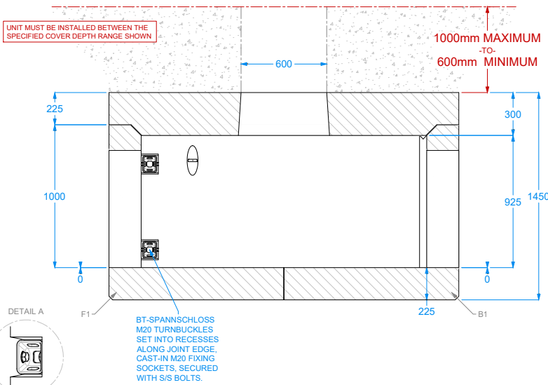
VIEW: SECTION X-X
